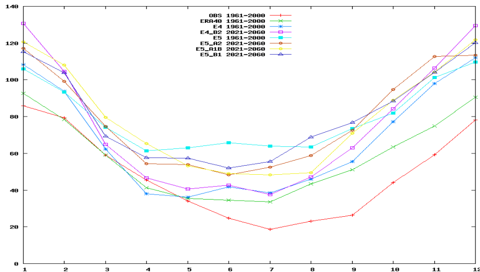
Figure 8: Annual cycle of observed and simulated (driven by ERA-40, ECHAM4 and ECHAM5 data) discharge, 1961-2000, compared with the simulated discharge for 2021-2060 driven by ECHAM4 and ECHAM5 data [ \text{m}^3/\text{s} ]
