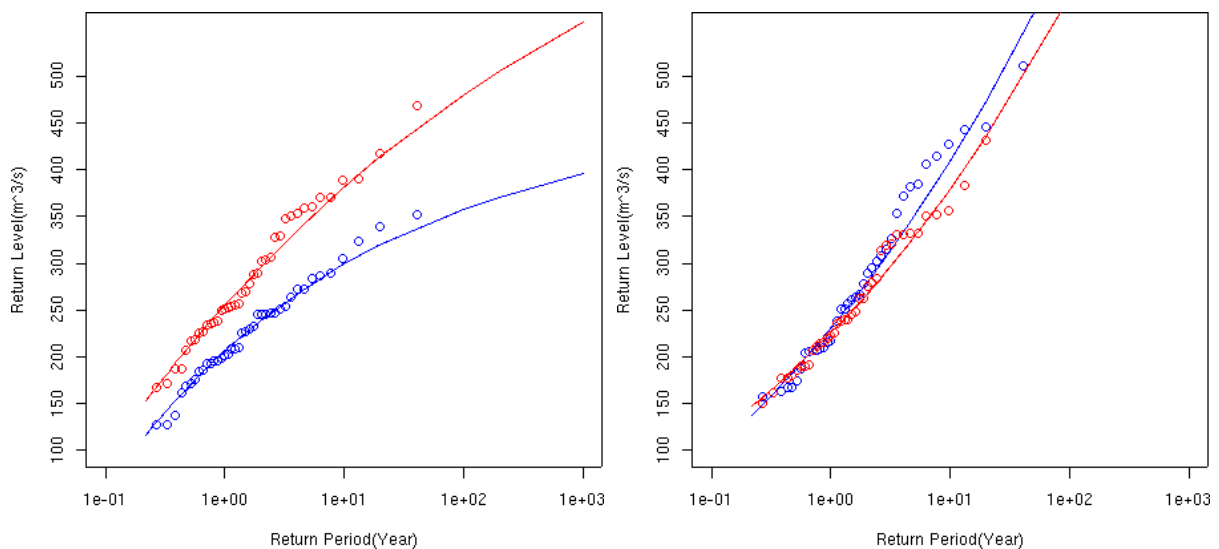
Figure 9: Return values of the simulated maximum annual discharge using the ECHAM4-B2 (a) and ECHAM5-A2 (b) driven RCA3 simulation for the present-day (blue) and future climate (red)
