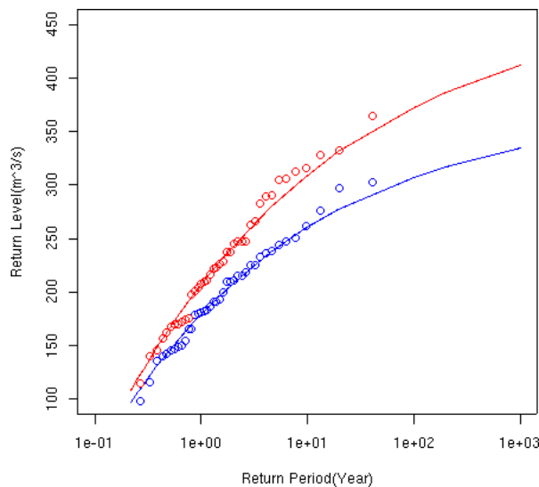
Figure 6: Return values of observed (red) and simulated (blue) (ERA-40 driven simulation) maximum annual discharge (Circles: Values of maximum daily discharge per year, lines: Fit using generalized extreme value distribution)
