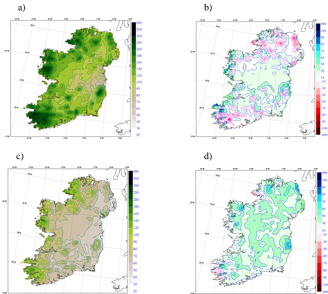
Figure 3: Mean monthly precipitation (1961-2000) from UKCIP data for January (a) and July (c) and differences of our ERA-40 driven RCA3 simulation relative to the UKCIP data ((b) and (d)) in mm/month. The UKCIP data are based on observed precipitation values interpolated to a 5-km grid.
