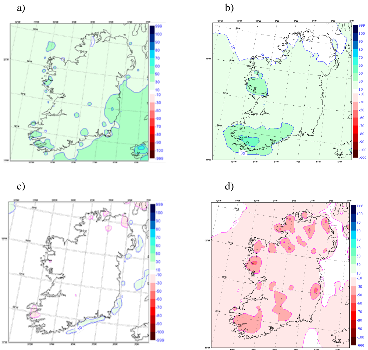
Figure 7: Predicted precipitation changes in mm/month in January according to (a) the ECHAM4-B2 scenario and (b) the ECHAM5-A1B scenario and in July according to (c) the ECHAM4-B2 scenario and (d) the ECHAM5-A1B scenario.
