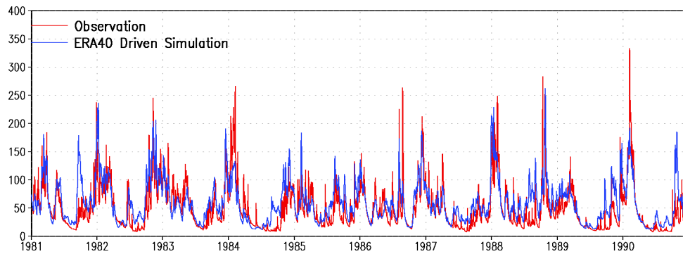
Figure 5: Observed and simulated (ERA-40 driven simulation) discharge [ \text{m}^3/\text{s} ]
