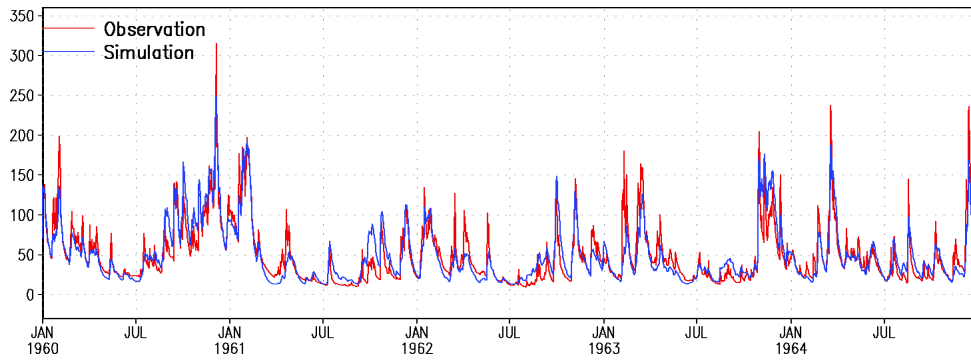
Figure 4: Observed and simulated (using observed precipitation as the input) discharge [ \text{m}^3/\text{s} ]
